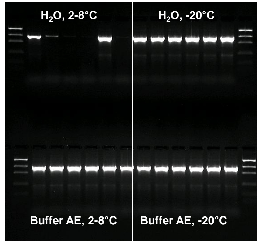
1 kb PCR amplicon on 1.0% agarose gel
