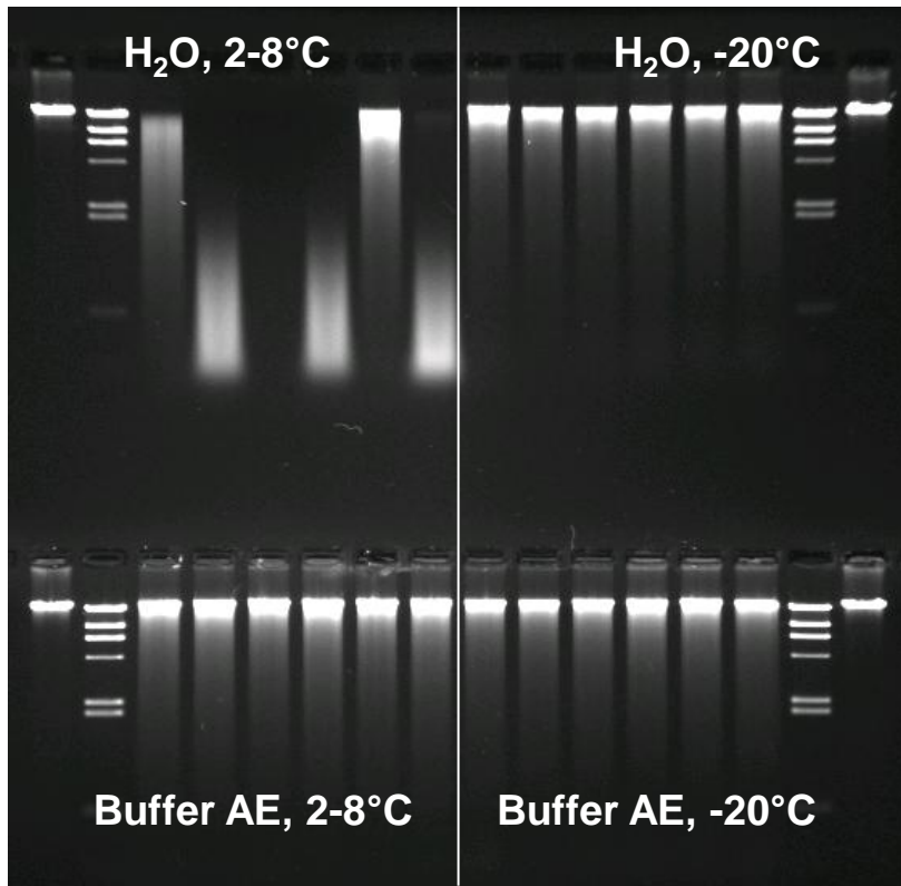
genomic DNA on 0.8% agarose gel
